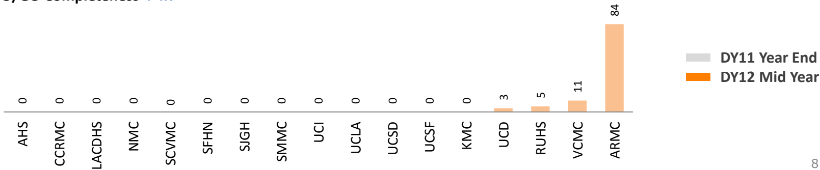
SO/GO Completeness P4R
